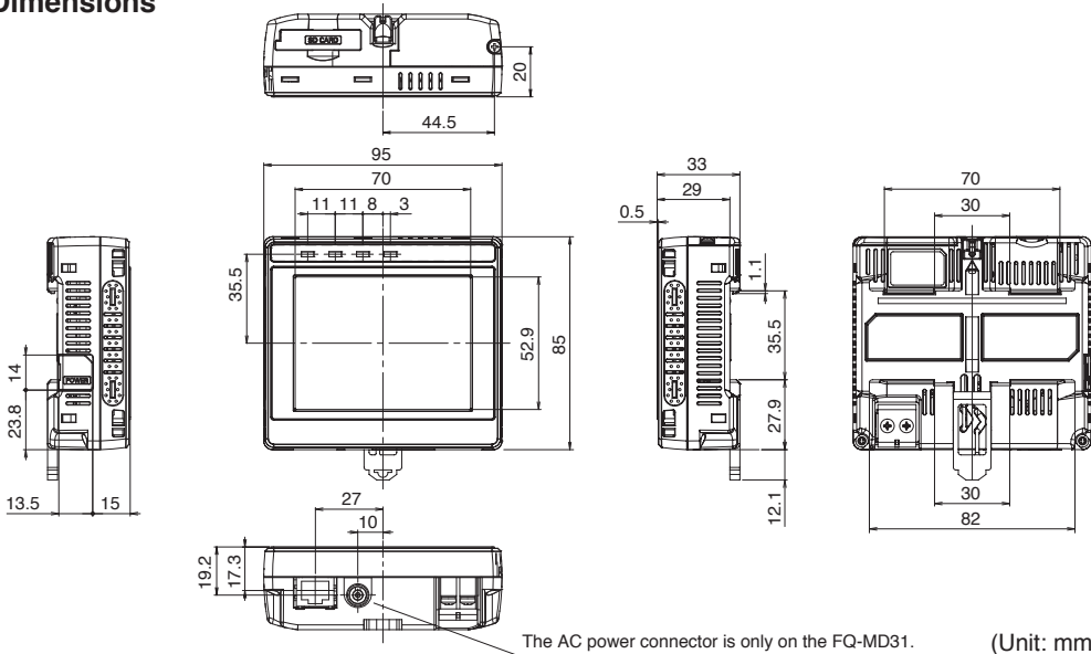
The AC power connector is only on the FQ-MD31. (Unit: mm)
